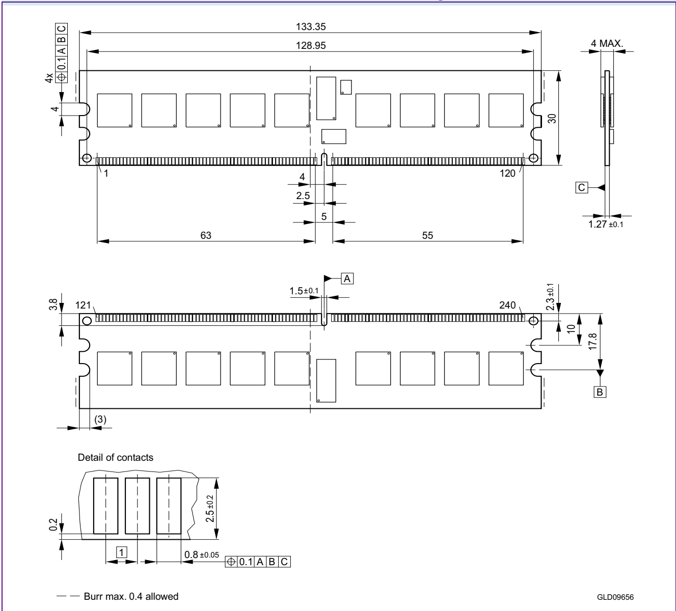
FIGURE 6 Package Outline Raw Card G L-DIM-240-12
